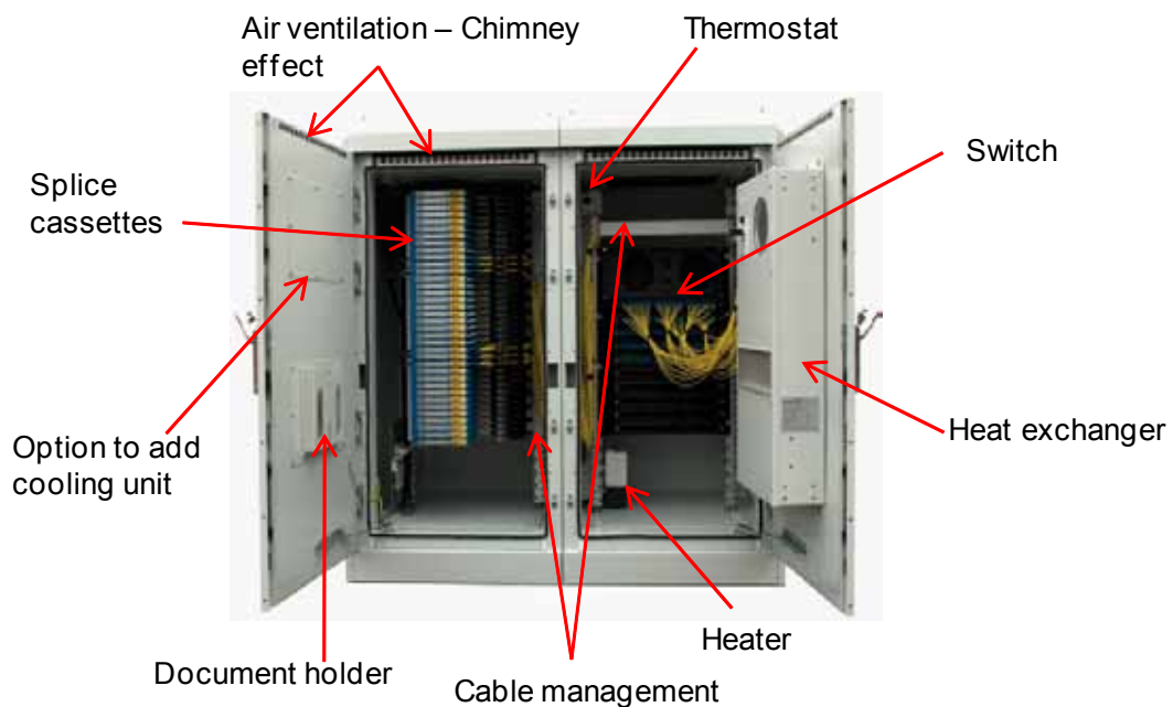
In-ground root double cabinet
